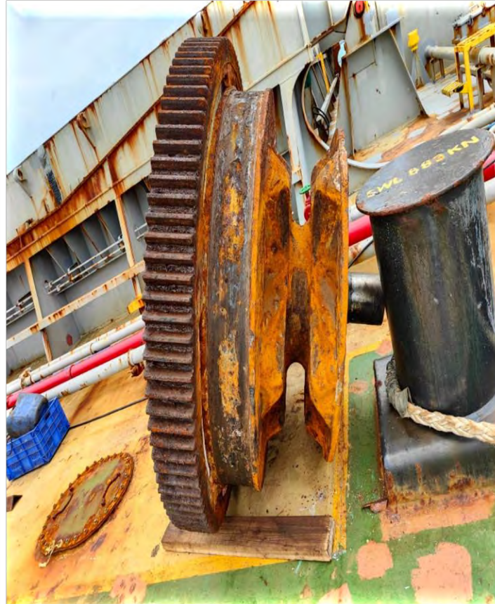
Mooring Winch Overhaul Vessel at Singapore Anchorage
